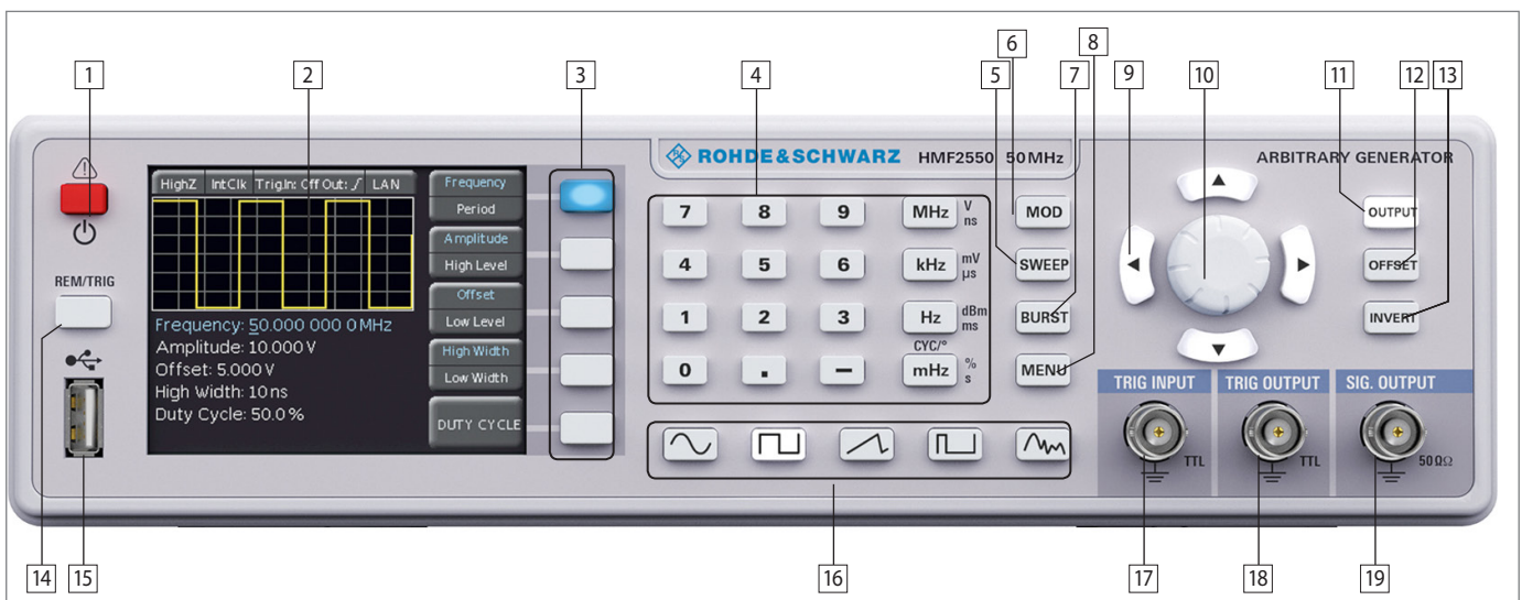
Fig. 2.1: Front panel of the HMF2550 / HMF25525
